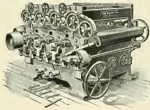
POWER FEED SANDER.
